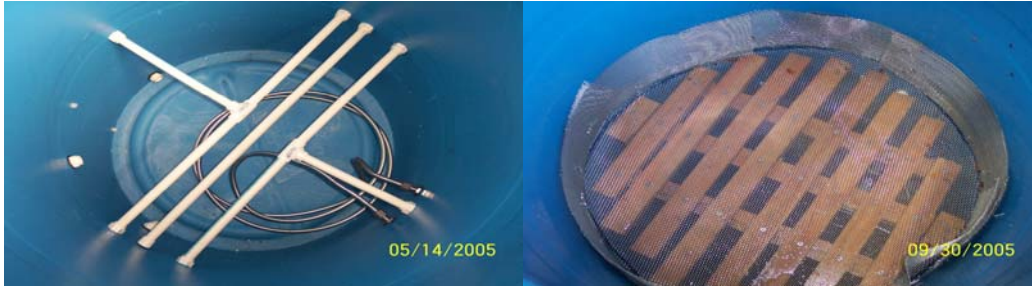
Figure 19: CPVC Pipes Support & Stainless Steel Mesh on Partition
