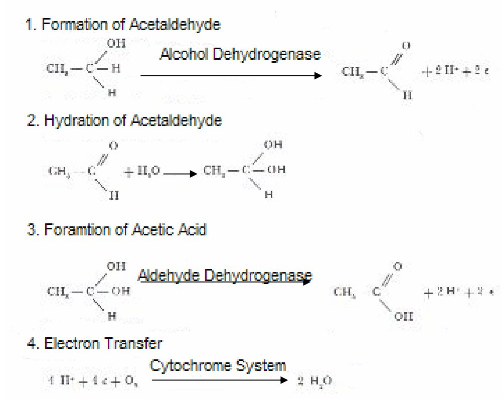
Figure 5: Conversion of Alcohol to Acetic Acid Reaction
