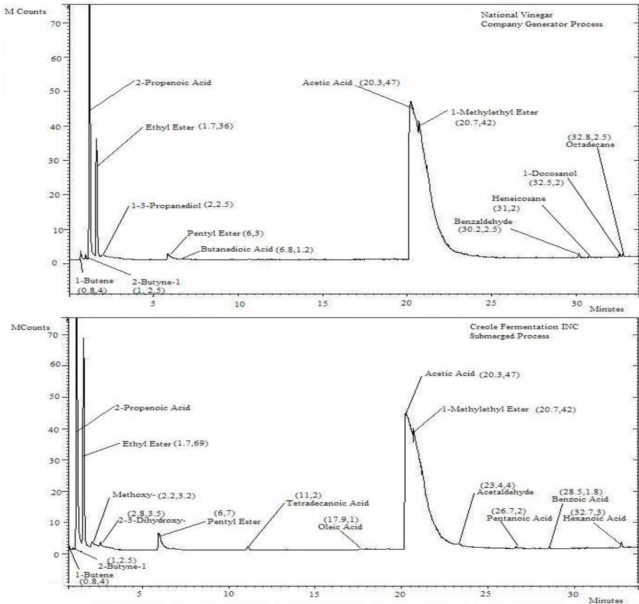
Figure 73: GC-MS Profiles of Vinegar from Commercial Generator and Submerged Processes
