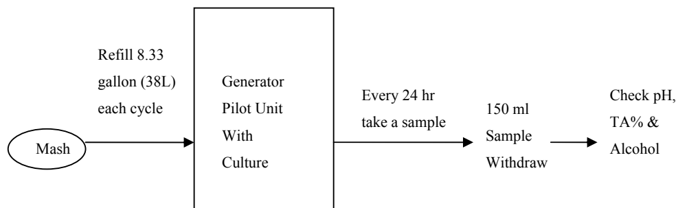
Figure 28: Generator Pilot Unit Flow Chart
