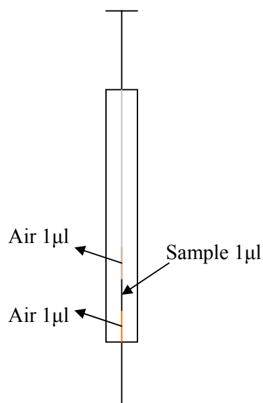
Figure 56: Injector Method
