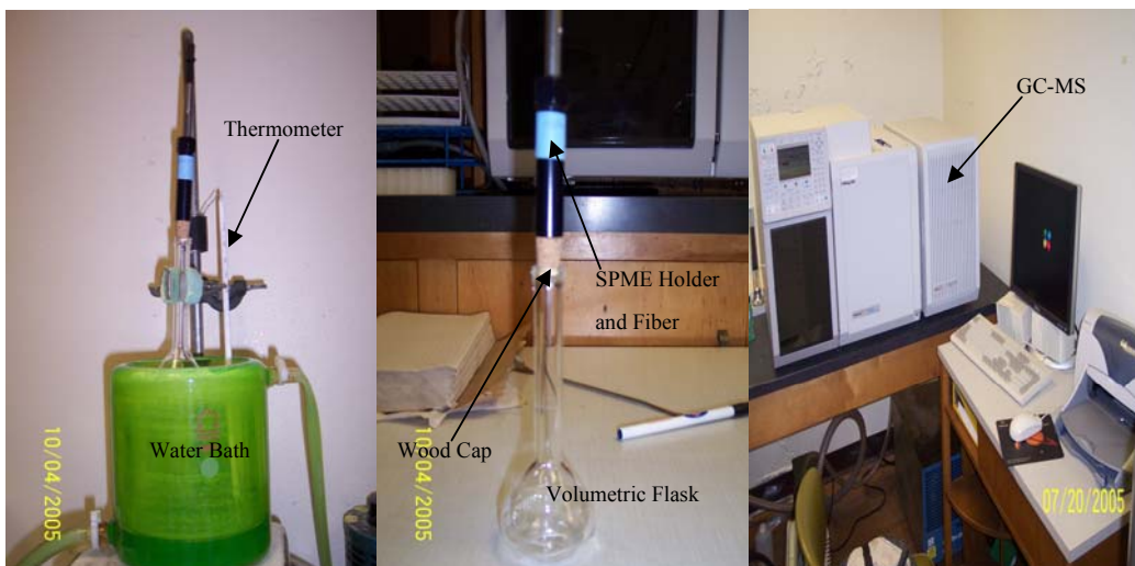
Figure 59: Water bath, SPME setup and GC-MS
