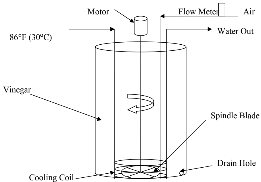
Figure 45: Submerged Acetification Process 2 Flow Chart
