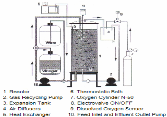
Figure 10: Semi-Continuous Process
