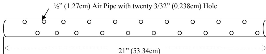
Figure 22: Air Pipe Drawing
