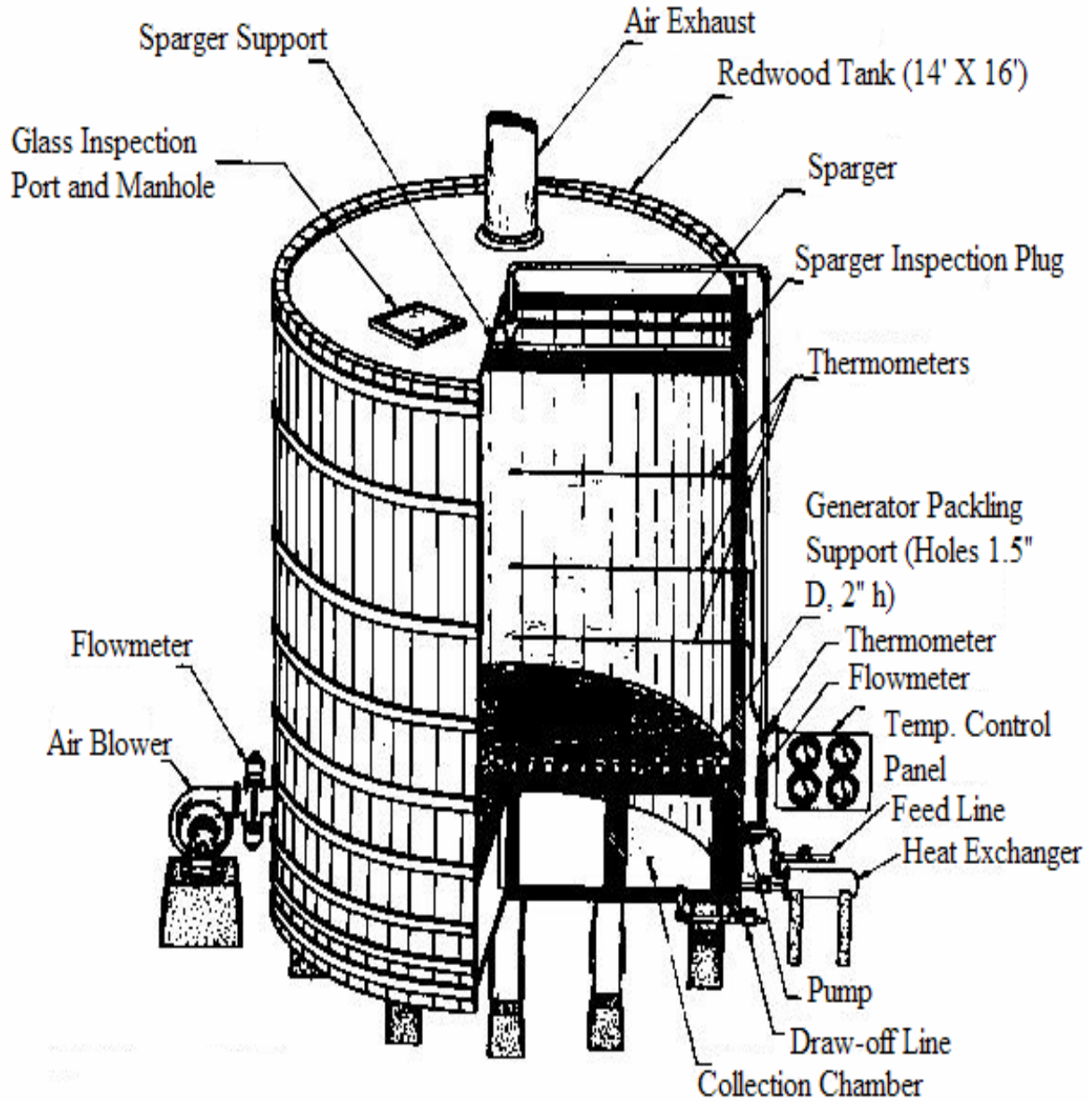
Figure 7: Vinegar Generator
