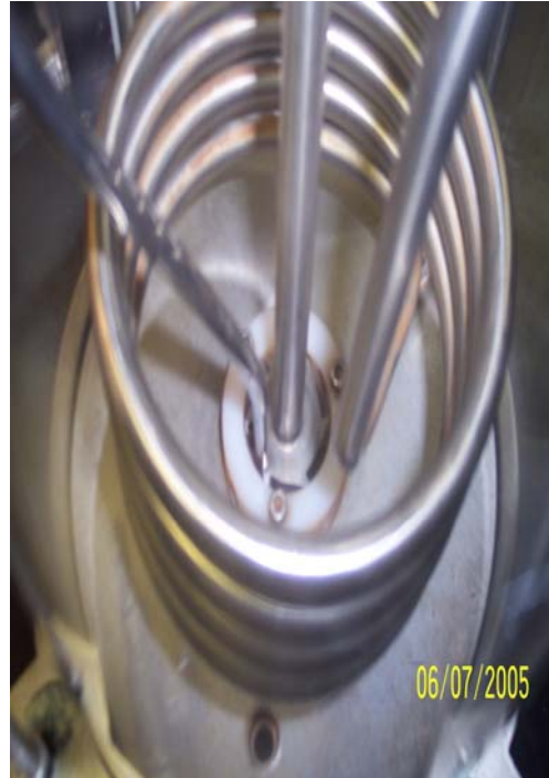
Figure 43: Aerator Sits on the Air Hole and Spins at 3450rpm
