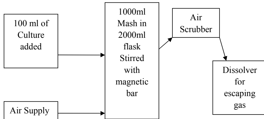
Figure 32: Submerged Process 1 Flow Chart
