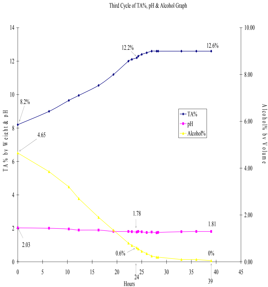
Figure 72: Third and Final Cycle – Submerged Process
